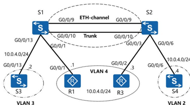
Figure 1.2 VLAN topology
